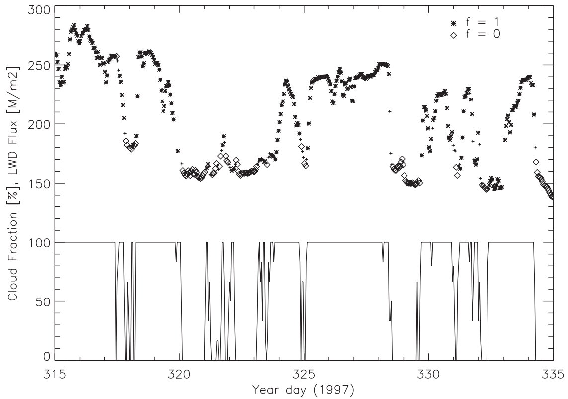
Figure 4. Time series of hourly averaged downward LW flux in W m^{-2} (upper panel) where asterisks correspond to overcast skies (cloud fraction = 1.0), diamonds to clear skies (cloud fraction = 0.0) and crosses otherwise. Corresponding time series of hourly averaged cloud fraction (lower panel).
